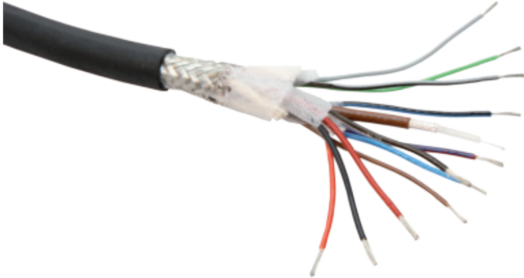
Cable section
